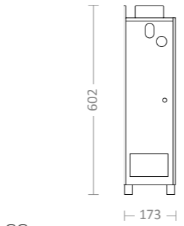
CC Coin Changer 17 kg
