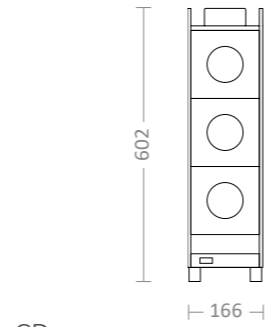
CD Cup Dispenser 13 kg
