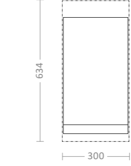
UBR / UBR-CF 10 l Refrigerator Under Counter 30 kg | 230 V | 0.1 kW
