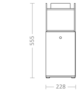
Lv Cup Warmer / 4 l Refrigerator 20 kg | 230 V | 0.16 kW
